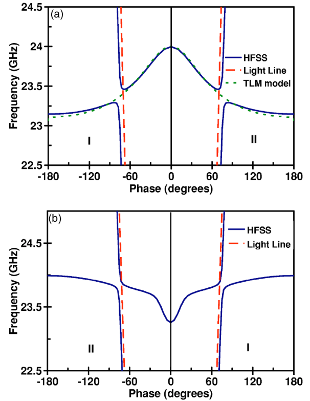
FIG. 5. (Color online) Dispersion plots for (a) OS structure and (b) SS structure. In the OS configuration the unit cell size was 2.5 \times 2.5 \times 2.5 mm. The unit cell size was 4 \times 2.5 \times 2.5 mm in the SS case.
